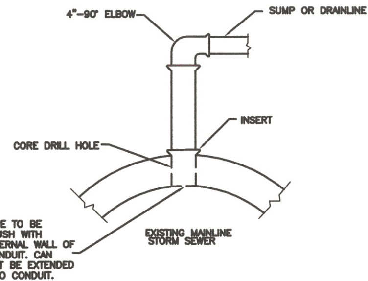
TYPICAL DIRECT CONNECTIONS (TO MAINLINE STORM SYSTEM) 12" OR LARGER
