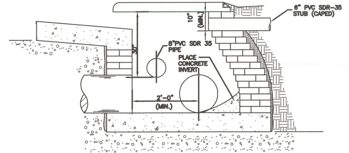
TYPICAL SECTION TIE INTO CATCH BASIN
